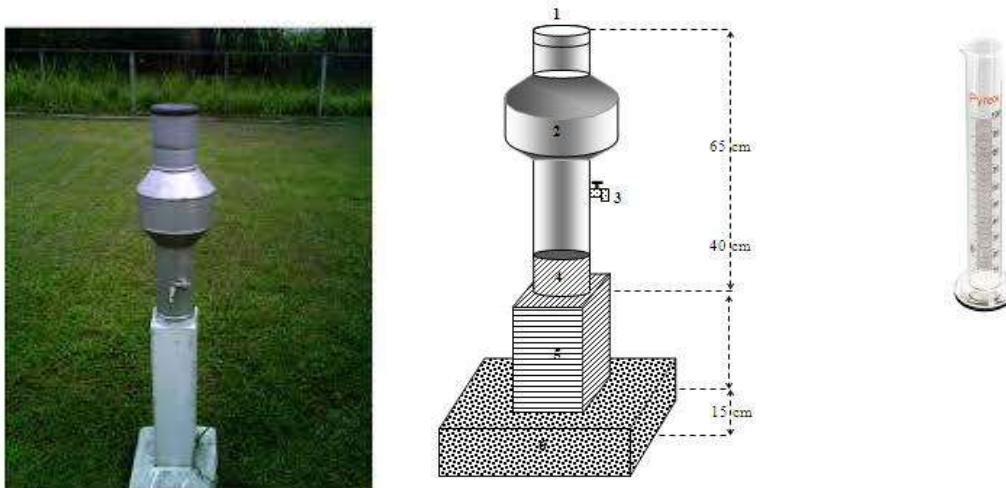
Gambar 3.1 Alat Penakar Hujan Manual (Ombrometer)
